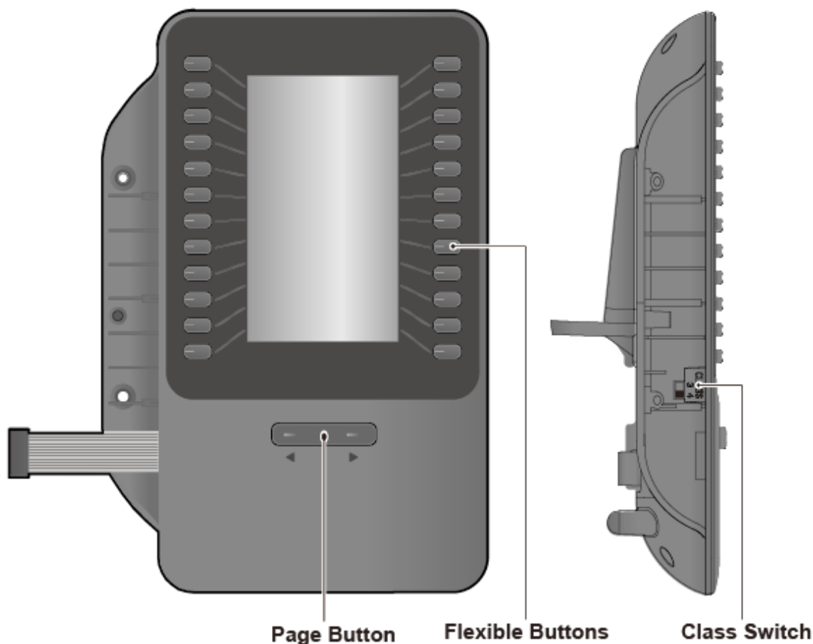
Figure 1.6-2: 1048ilss
