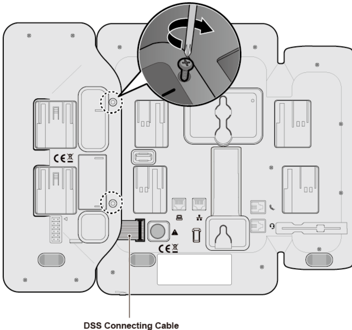
Figure 1.6-3: 1024idss Installation
