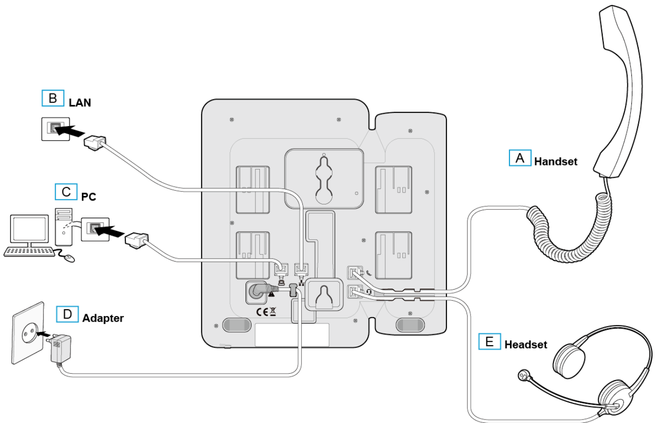
Figure 1.5: 1000i Installation
