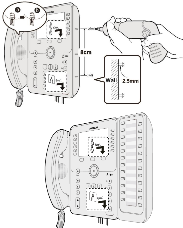
Figure 1.7_Wall Mount
